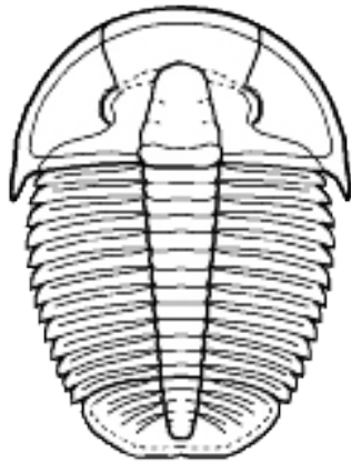
Triassic period
